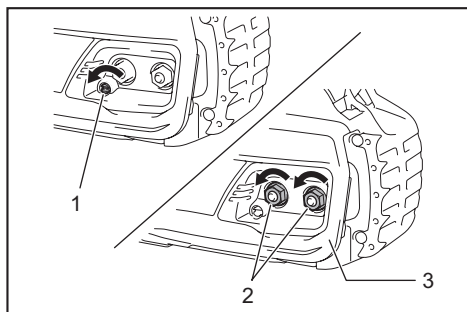
► 1. Chain adjusting screw 2. Retaining nut 3. Sprocket cover
