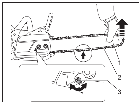
► 1. Guide bar 2. Saw chain 3. Chain adjusting screw
